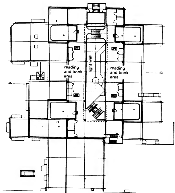
⑥ Second floor
